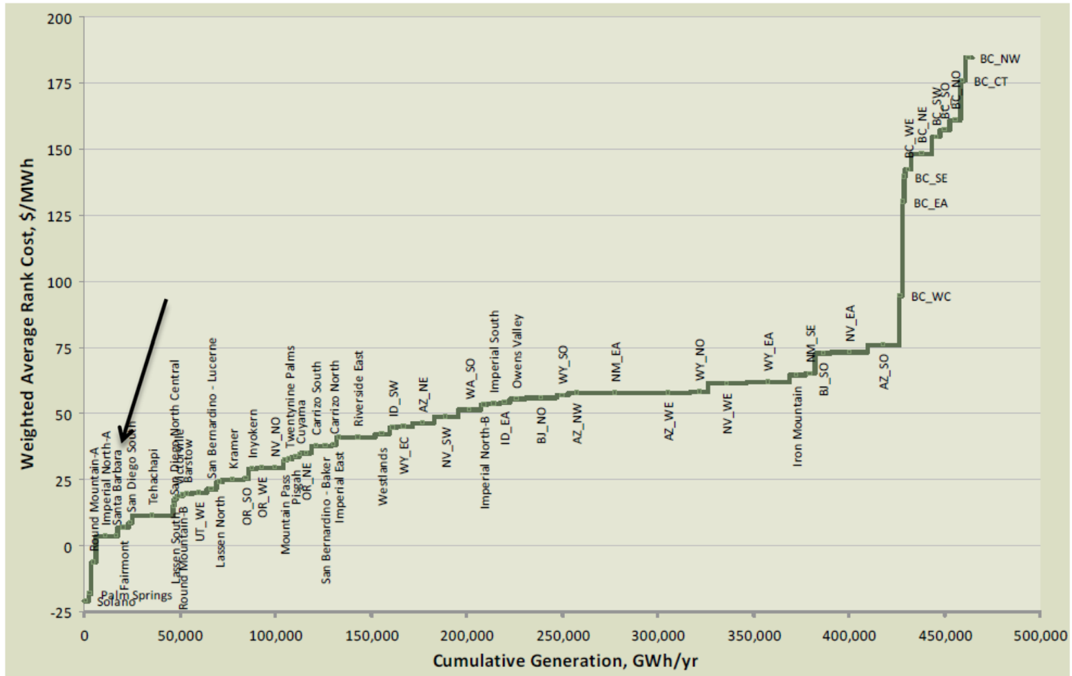
Figure 1-3. Weighted Average Rank Cost (2010 $/MWh) for CREZs.
