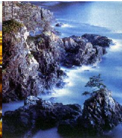
Figure 16: Natural processes are continually reshaping coastal areas where oceans meet land.
